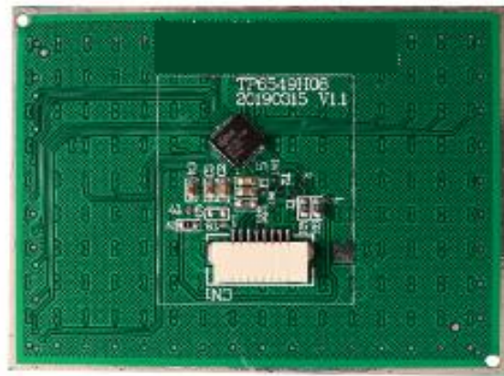
Back view of the item
